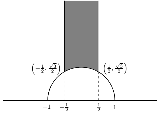
Fig. 1.1: A fundamental domain E \subseteq \mathbb{H} for the action of \mathrm{SL}_2(\mathbb{Z}) .
