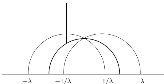
Fig. 1.4: The union of the two geodesics considered in X_2 with both directions allowed is a periodic A -orbit, and comprises the orbit SL_2(\mathbb{Z})g_{\text{golden}}A .
