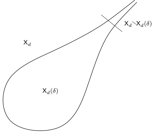
Fig. 1.8: A compact subset of X_d is contained in X_d(\delta) = \{A \in X_d \mid \lambda_1(A) \geq \delta\} for some \delta > 0 . The non-compact part X_d \setminus X_d(\delta) , loosely referred to as a cusp , is depicted as a thin set to indicate the finite total volume (see Theorem 1.51). For d > 2 the geometry of the cusp is much more complicated than the cusp in the d = 2 case.
