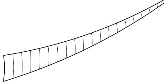
Fig. 1.2: Folding the hyperbolic triangle in Figure 1.1 creates a surface stretching off to infinity (the cusp) and with two exceptional points (with conical singularities).
