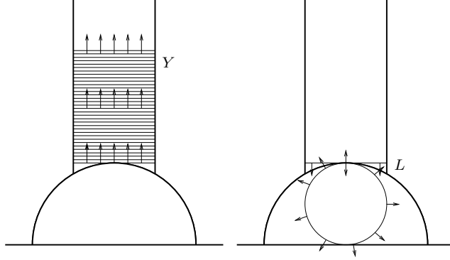
Fig. 1.6: The set Y on the left is a cylinder within the three-dimensional quotient \mathbf{X}_2 . The set L on the right can be drawn outside of F using a circle tangent to \mathbb{R} at 0 or inside of F using a horizontal line with arrows pointing downwards. Note that L and Y intersect only at (i, \uparrow) .
