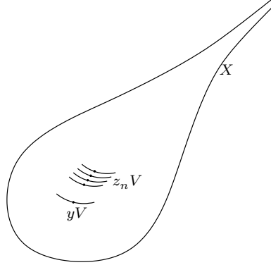
Fig. 1.7: We depict here an alternative to the proof of Corollary 1.33: By assuming (for the purposes of a contradiction) that the sets z_n V \subseteq xH approach yV \subseteq xH transverse to the orbit direction for a given neighbourhood V of e \in H , one can show that \text{vol}(xH) = \infty .
