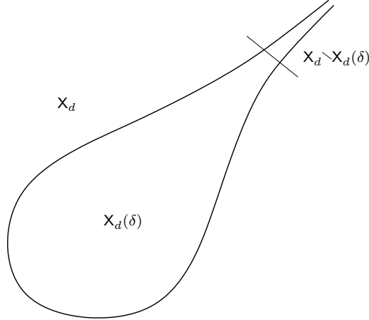
Fig. 1.10: A compact subset of \mathbf{X}_d is contained in \mathbf{X}_d(\delta) = \{A \in \mathbf{X}_d \mid \lambda_1(A) \geq \delta\} for some \delta > 0 . The non-compact part \mathbf{X}_d \setminus \mathbf{X}_d(\delta) , loosely referred to as a cusp , is depicted as a thin set to indicate the finite total volume (see Theorem 1.54). For d > 2 the geometry of the cusp is much more complicated than the cusp in the d = 2 case.
